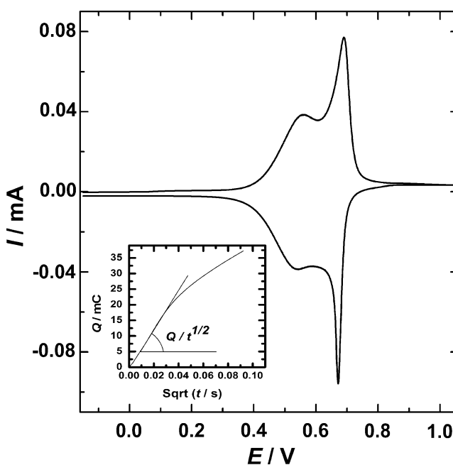
Fig. 2 Cyclic voltammetric response of NiHCF film on glassy carbon electrode recorded in 0.5 mol dm -3 K 2 SO 4 . Scan rate, 50 mV s -1 . Inset illustrates chronocoulometric response obtained upon application of the anodic potential step from 0 to 0.85 V
